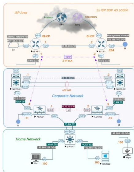
Dual ISP ASAv FW POC Lab Created by Uldis, EVE Pro, 2025
